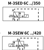
M-3SED 6C ../350
