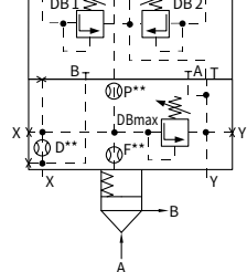
L-LFA...DBU3D.-7X/... Nominal sizes 80 and 100
