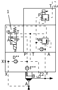
LFA..DREWW-7X/006 NG 25, 32
