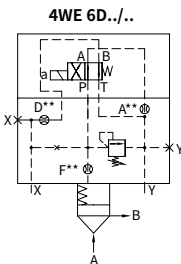
L-LFA...DBW..-7X/.. Nominal sizes 40, 50 and 63
