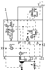
LFA..DREWZ-7X/014 NG 25, 32
