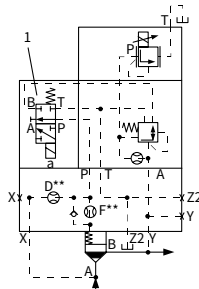
LFA..DREWW-7X/006 NG 40, 50
