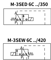
M-3SED 6C ../350
