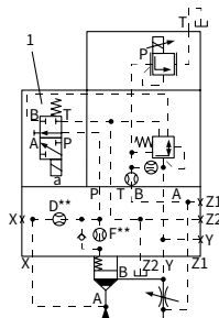
LFA..DREWZ-7X/014 NG 40, 50
