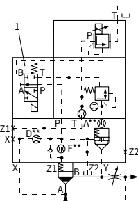
LFA..DREWZ-7X/014 NG 63
